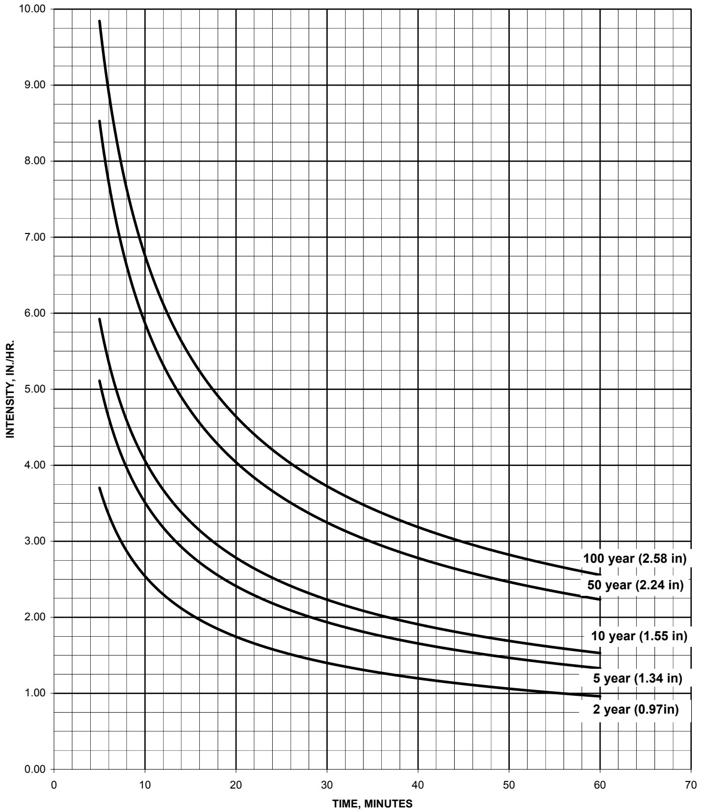
Figure 5-1 Flood Flows Time-Intensity-Frequency Curves
